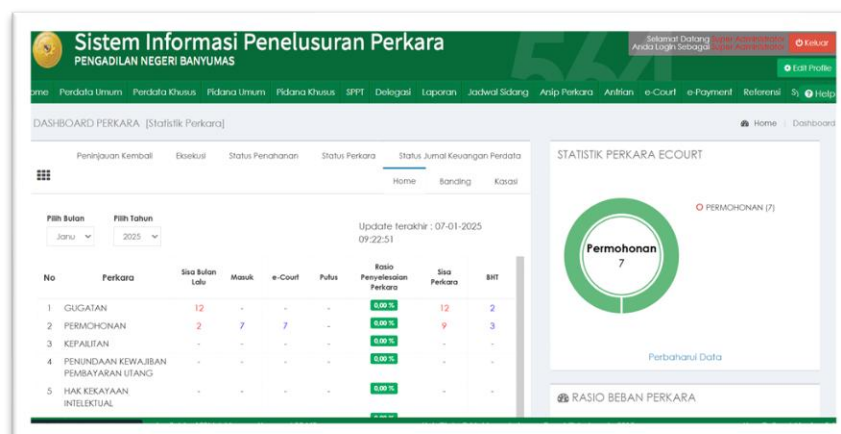
Gambar 4.3 Implementasi SIPP
